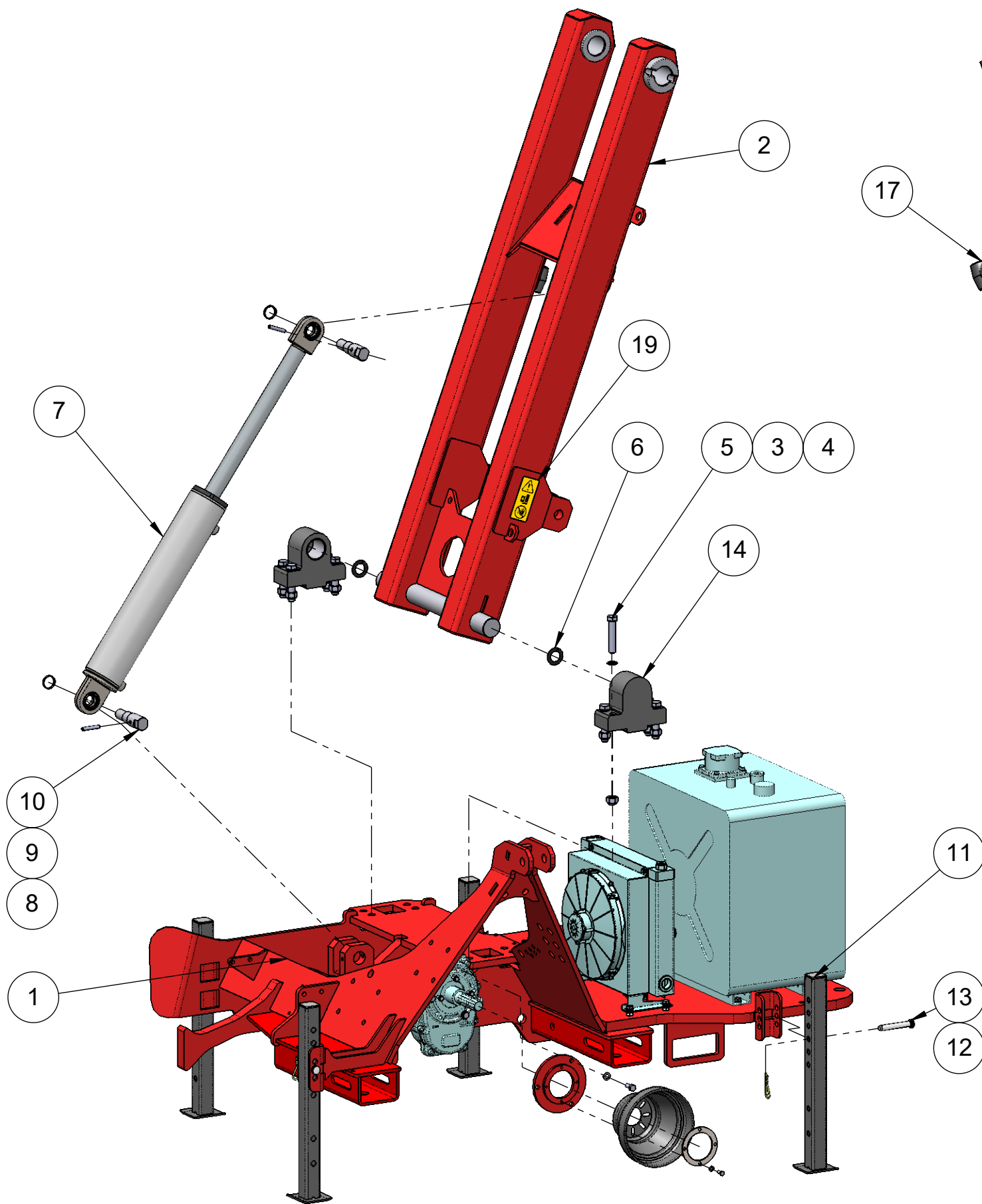
DETAIL A SCALE 1 : 15
